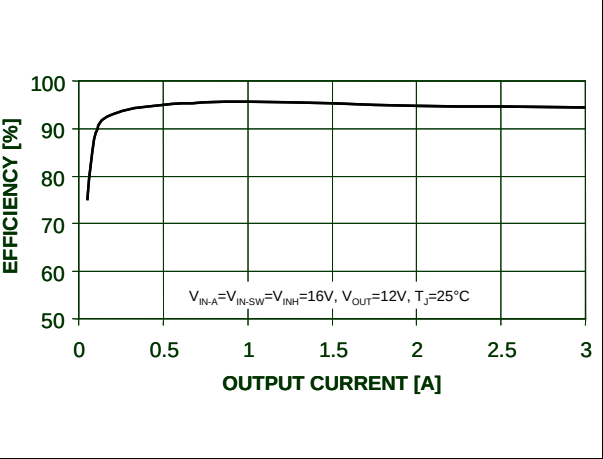
Figure 22. Efficiency vs. output current at V_{out} = 12V
