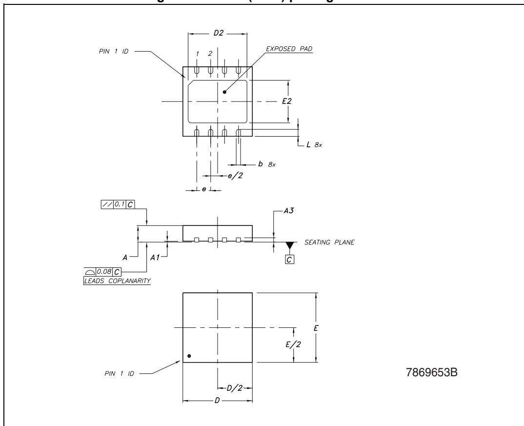
Figure 26. DFN8 (4 x 4) package outline
