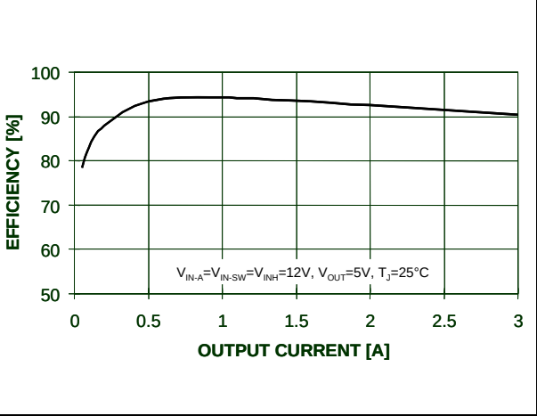
Figure 20. Efficiency vs. output current at V_{out} = 5V
