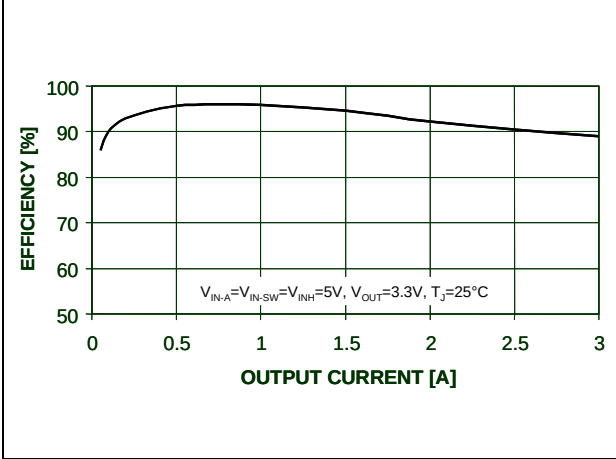
Figure 21. Efficiency vs. output current at V_{out} = 3.3V
