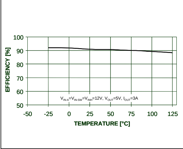
Figure 19. Efficiency vs. temperature
