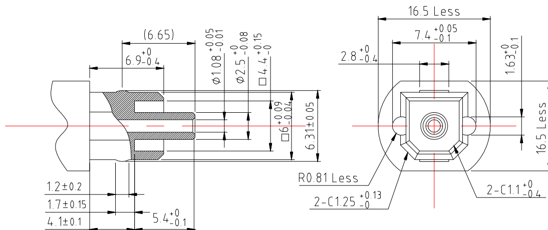
Fig.4 Adapted plug
