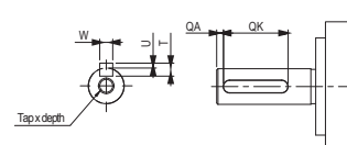
Shaft end
