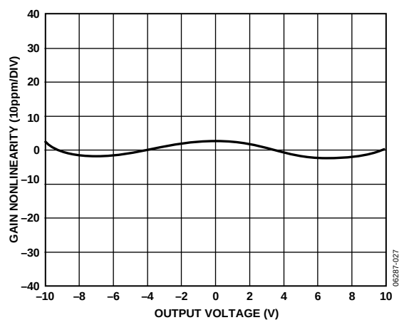
Figure 26. Gain Nonlinearity vs. Output Voltage, G = 8 , R_L = 10\text{ k}\Omega , 2\text{ k}\Omega , 600\text{ }\Omega
