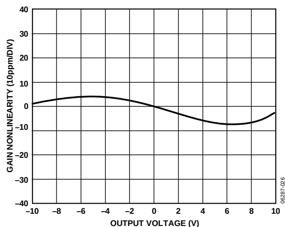
Figure 25. Gain Nonlinearity vs. Output Voltage, G = 4 , R_L = 10\text{ k}\Omega , 2\text{ k}\Omega , 600\text{ }\Omega
