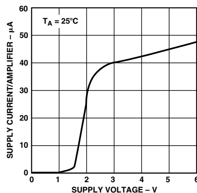
TPC 27. Supply Current per Amplifier vs. Supply Voltage
