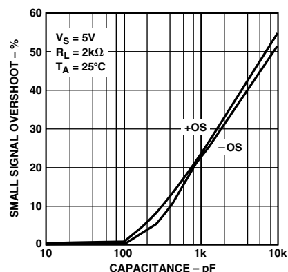
TPC 21. Small Signal Overshoot vs. Load Capacitance
