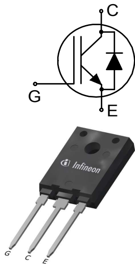
Fully isolated package TO-247
