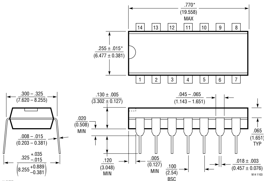
N Package 14-Lead PDIP (Narrow 0.300) (LTC DWG # 05-08-1510)
