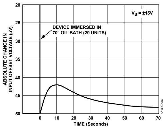
Figure 9. Offset Voltage Change Due to Thermal Shock
