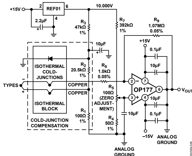
Figure 26. Thermocouple Amplifier with Cold Junction Compensation
