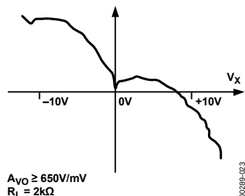
Figure 23. Typical Precision Op Amp
