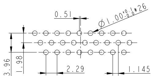
26 Pin Female connector PCB Pin Layout Scale 2:1
