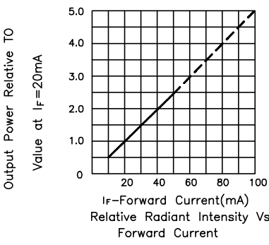
Relative Radiant Intensity Vs. Forward Current
