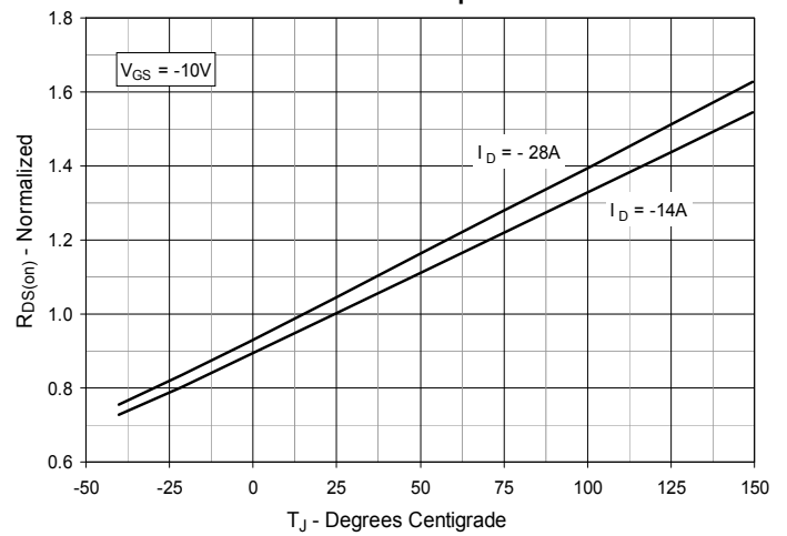
Fig. 4. R_{DS(on)} Normalized to I_D = -14A Value vs. Junction Temperature
