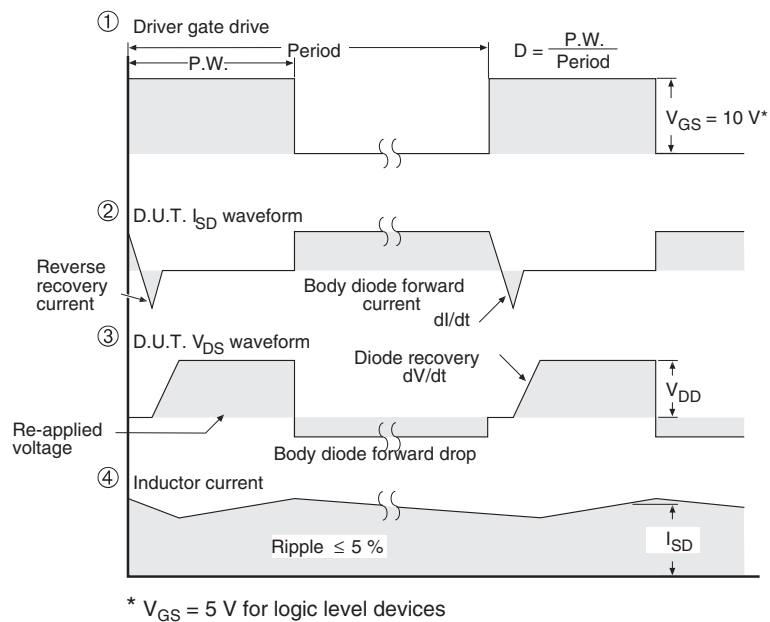
Fig. 11 - For N-Channel
