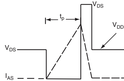
Fig. 9b - Unclamped Inductive Waveforms
