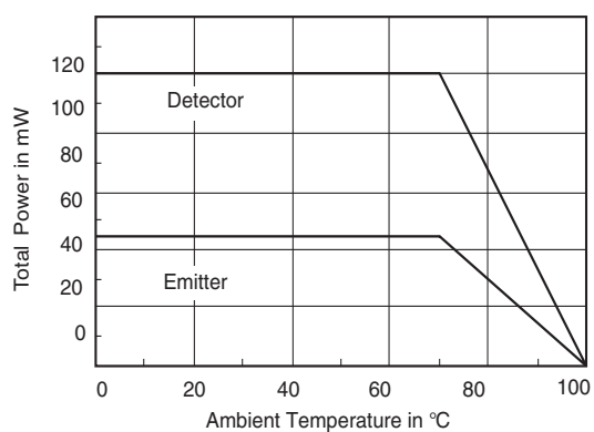
Figure 5. Permissible Power Dissipation vs. Temperature
