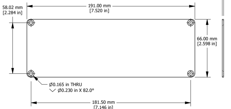
OPTIONAL FLANGED END PANELS 1455UF
