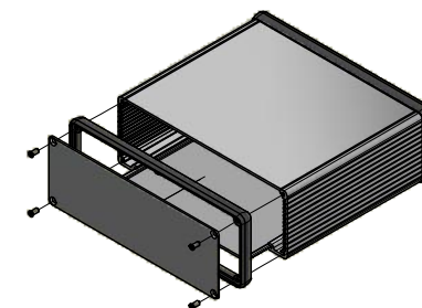
EXPLODED ISOMETRIC VIEW
