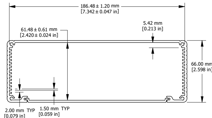
EXTRUSION
