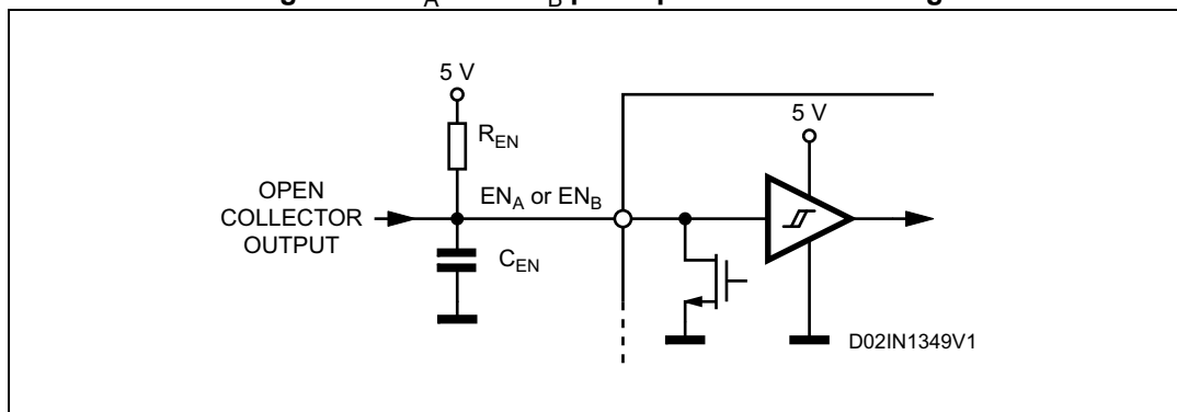
Figure 7. EN_A and EN_B pins open collector driving
