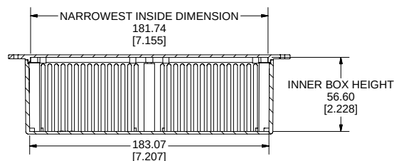
SECTION C-C
