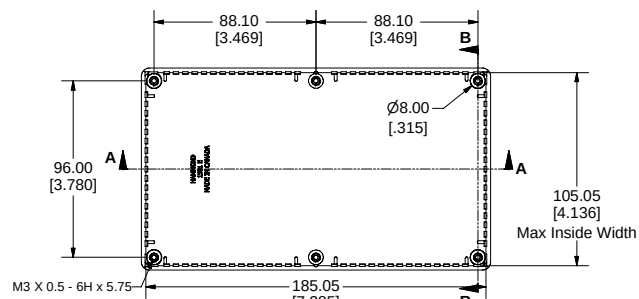
TOP VIEW OF BOX
