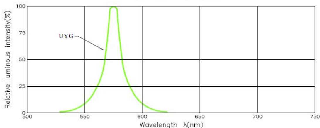
Spectrum Distribution
