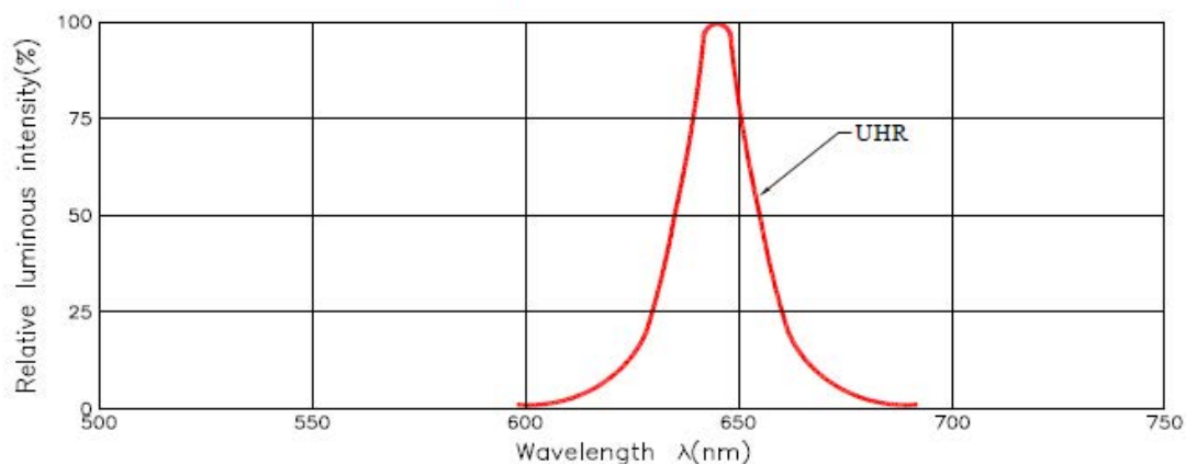
Spectrum Distribution
