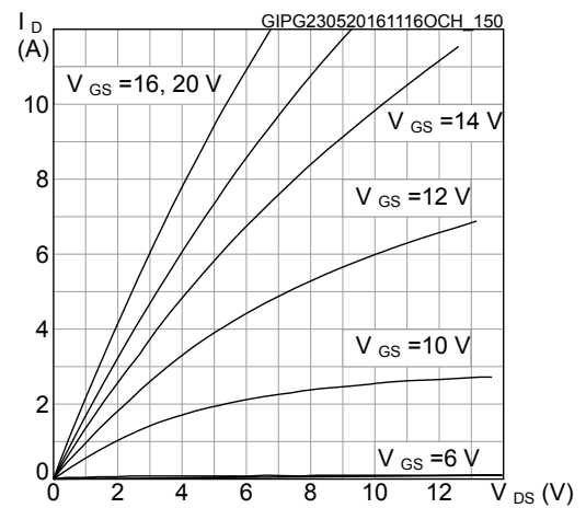
Figure 4. Output characteristics ( T_J = 150^\circ C )
