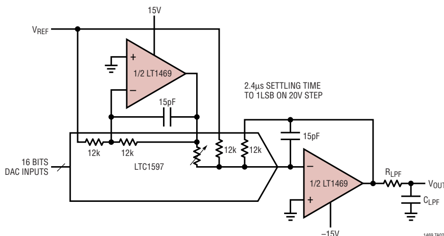
16-Bit DAC I-to-V Converter and Reference Inverter for Bipolar Output Swing ( V_{OUT} = -10\text{V} to 10\text{V} )
