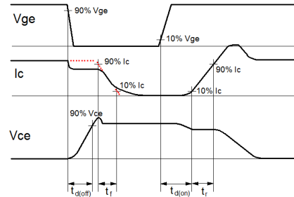
Inductive Switching Test Circuit & Waveforms
