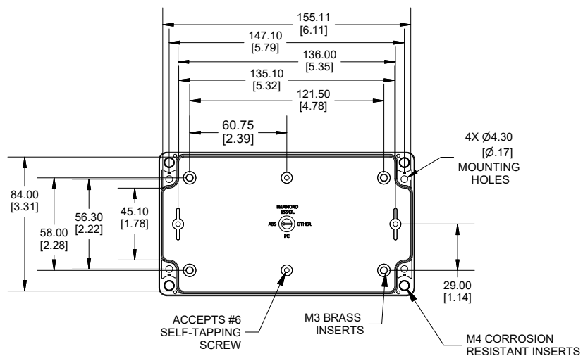
INSIDE BOX
