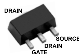
TO-243AA (SOT-89)
