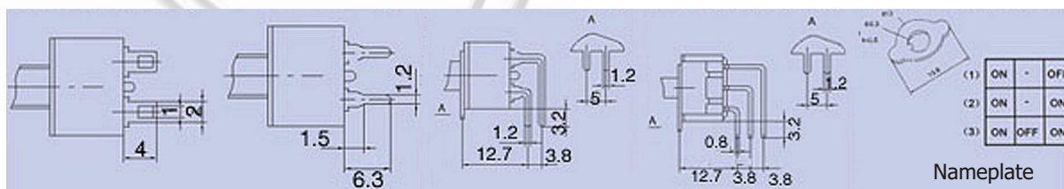
Solder terminal (1)
