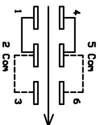
CIRCUIT: DPDT CONTACT CONFIGURATION
