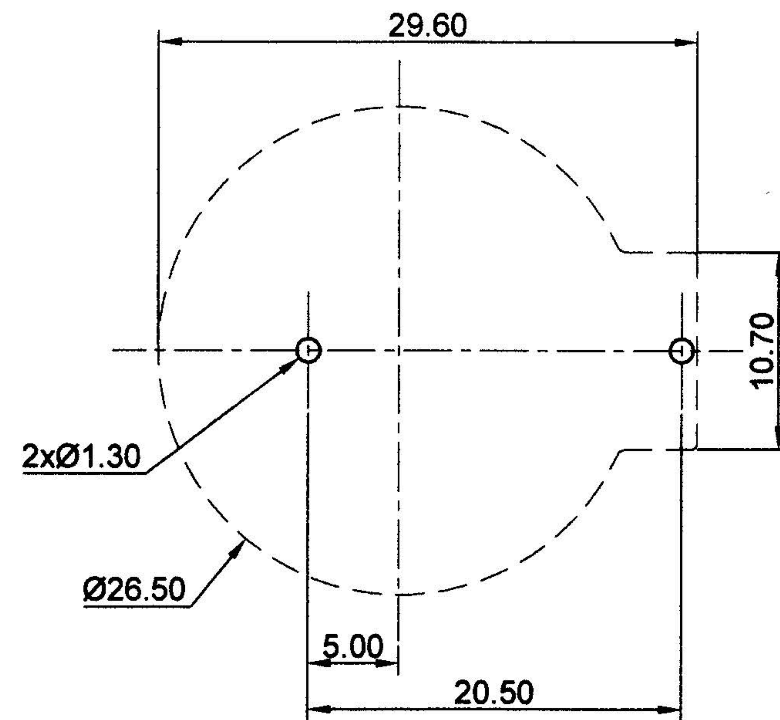
PCB MOUNTING LAYOUT
