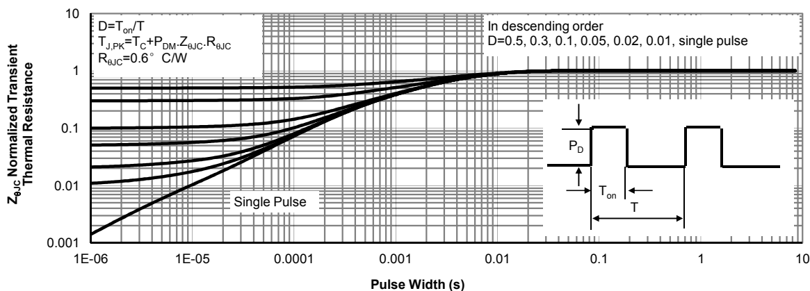
Figure 11: Normalized Maximum Transient Thermal Impedance for AOT20N25 (Note F)
