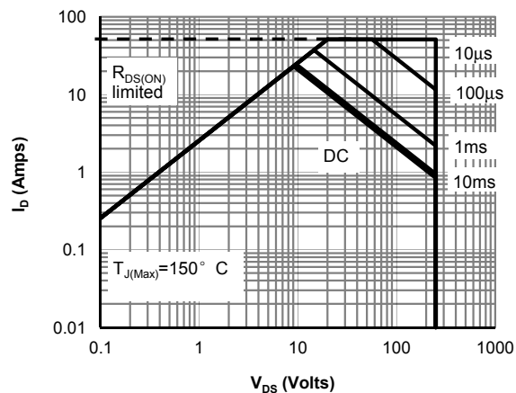
Figure 10: Maximum Forward Biased Safe Operating Area for AOT20N25 (Note F)
