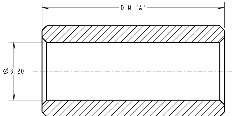
SECTION X-X
