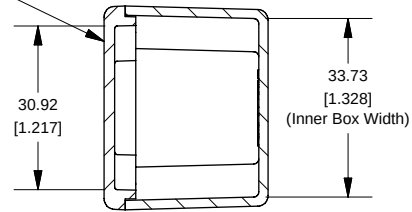
SECTION A-A End View of Assembly
