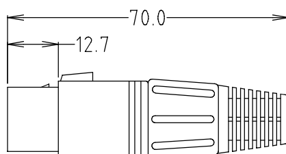
FC6180 - 7 PIN MALE PLUG 7APM/M
