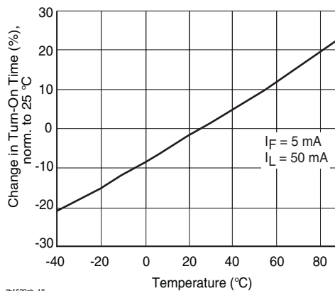
Figure 19. Turn-on Time vs. Temperature
