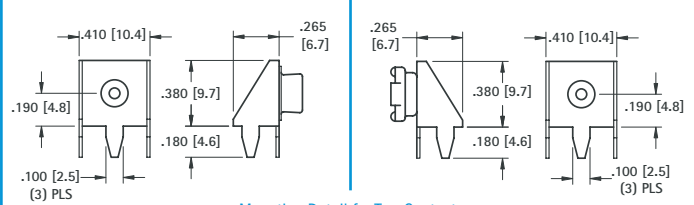
Mounting Detail for Two Contacts
