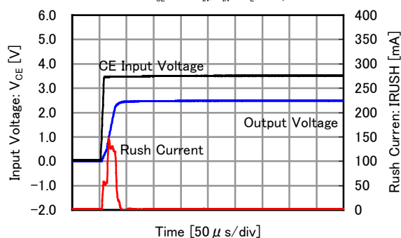
XC6223x251
