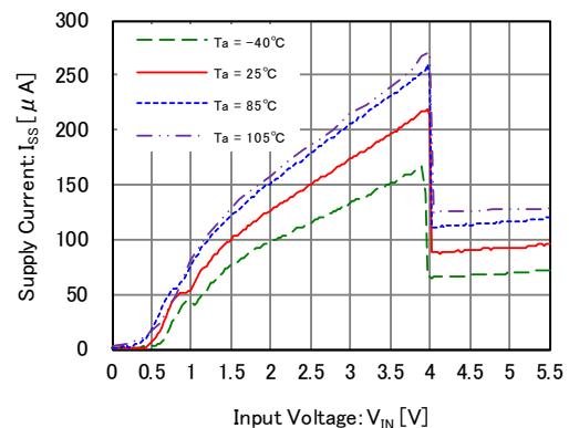
XC6223x401
