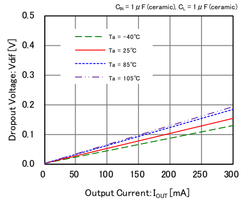
XC6223x401
