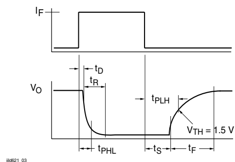
Figure 3. Saturated Switching Timing
