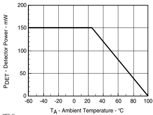
Figure 11. Maximum Detector Power Dissipation
