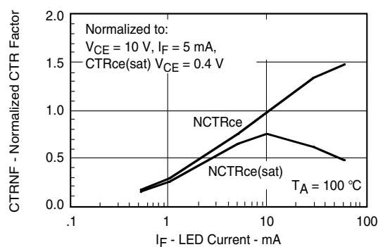
Figure 14. Normalization Factor for Non-saturated and Saturated CTR vs. I_F
