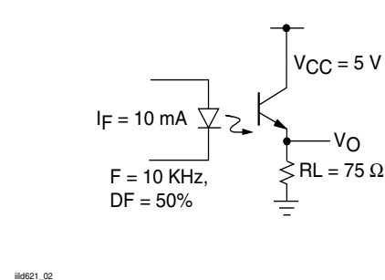
Figure 2. Non-saturated Switching Timing
