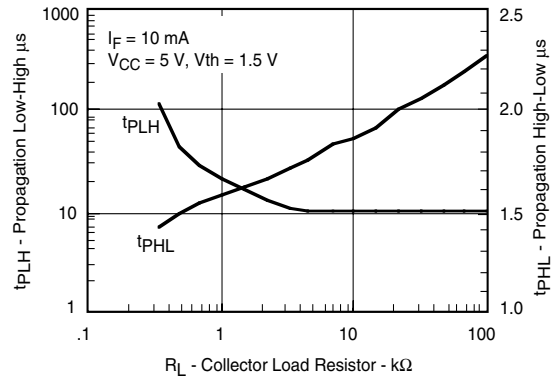
Figure 10. Propagation Delay vs. Collector Load Resistor
