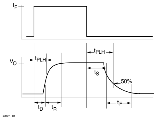
Figure 1. Non-saturated Switching Timing
