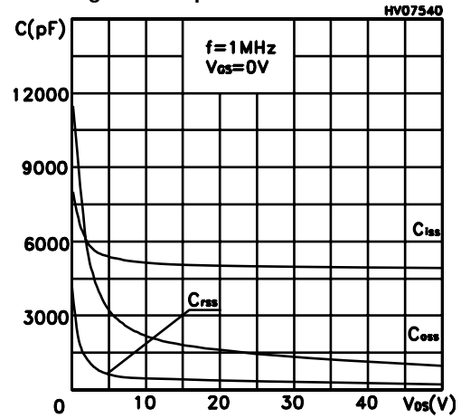
Figure 9: Capacitance variations
