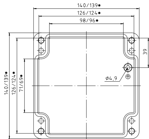
Deckel
