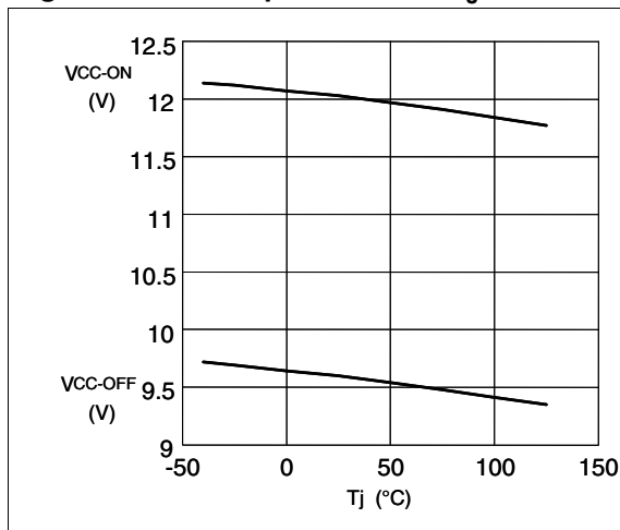
Figure 8. Start-up & UVLO vs T_j
