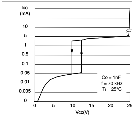
Figure 4. Supply current vs supply voltage
