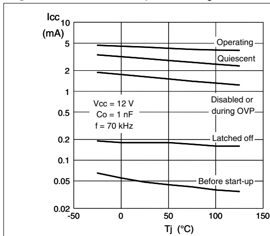
Figure 6. IC consumption vs T_j
