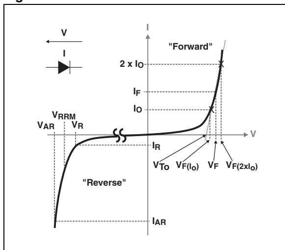
Figure 1. Electrical characteristics(a)
