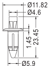
MOUNTING HOLE Ø6.3 THICKNESS 7.0
