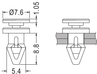
HOLE IN FAN Ø4.4 THICKNESS 3.0
