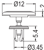
MOUNTING HOLE Ø3.5 THICKNESS 1.6~2.4
