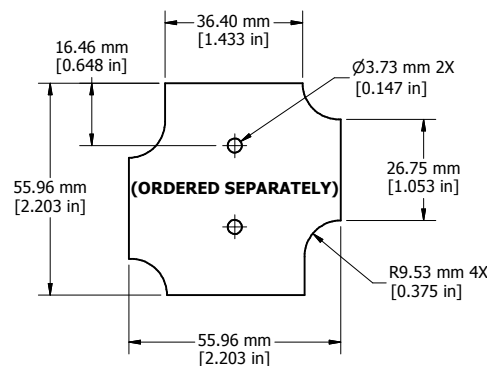
STEEL INNER PANEL
