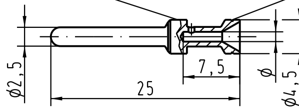
Stiftkontakt male contact
