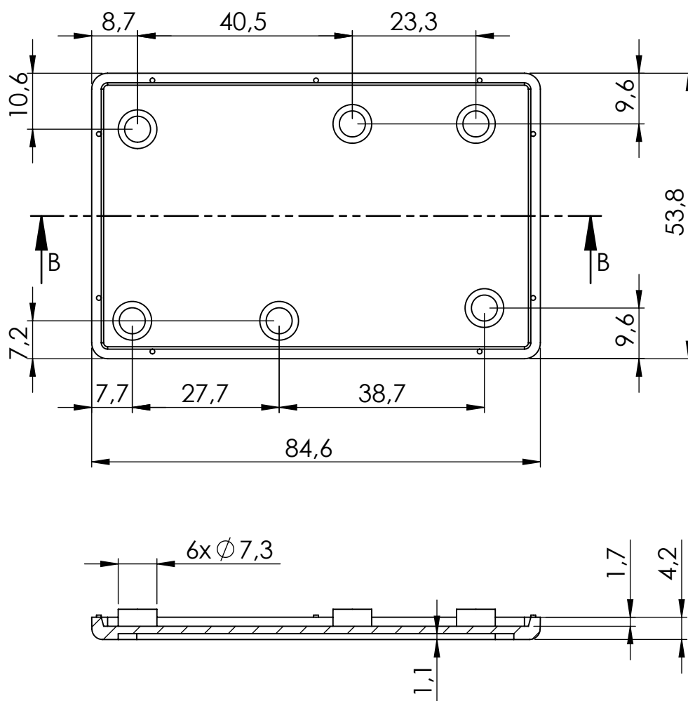
SECTION B-B
