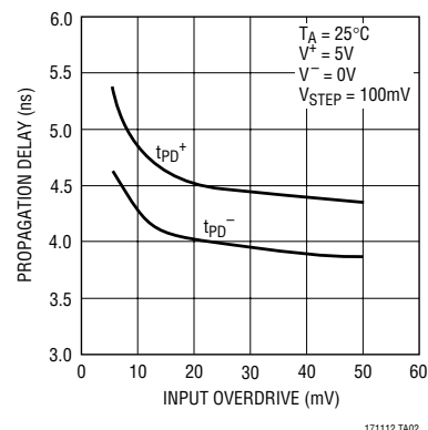
LT1711/LT1712 Propagation Delay vs Input Overdrive
