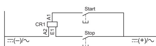
Pushbutton control
