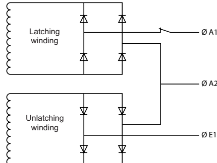
Scheme of internal circuit
