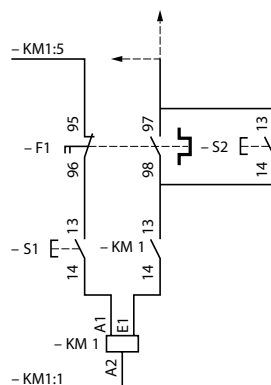
Contactors CR1 F
