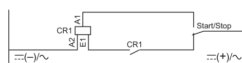
Switch control
