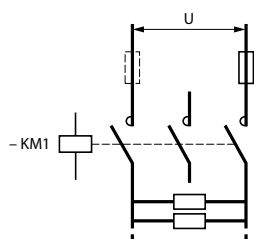
Circuit controlled by 2 poles of the contactor.
