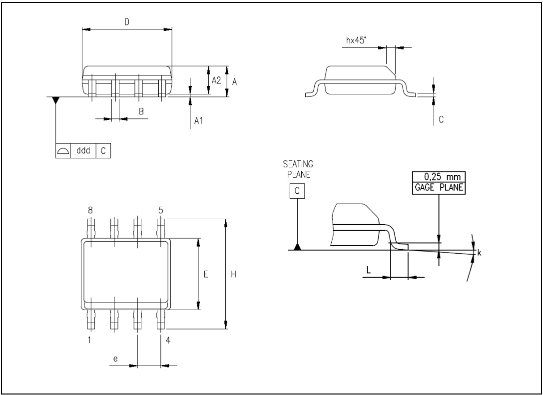
Figure 17. Package dimensions
