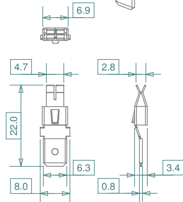
Tab contact (used in H1110)
