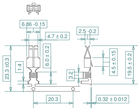
Crimp contact
