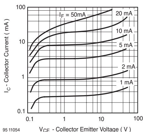
Figure 12. Collector Current vs. Collector Emitter Voltage
