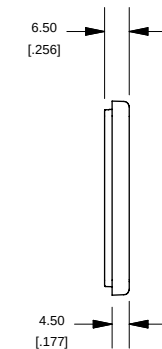
SIDE VIEW OF LID
