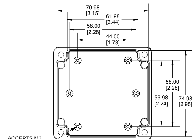
INSIDE BOX
