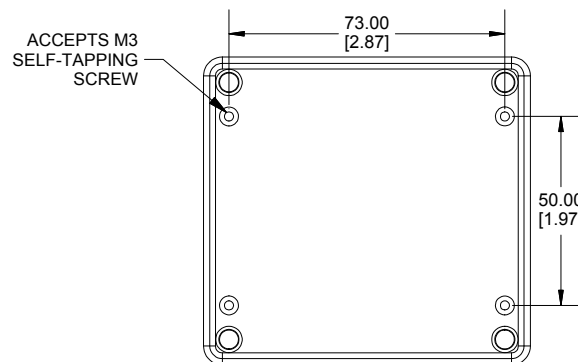
MOUNTING HOLES
