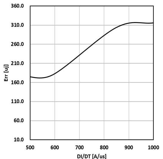
Figure 16. Typical diode Err vs di/dt Tc=25°C VCC=400V VGE=15V IF=40A
