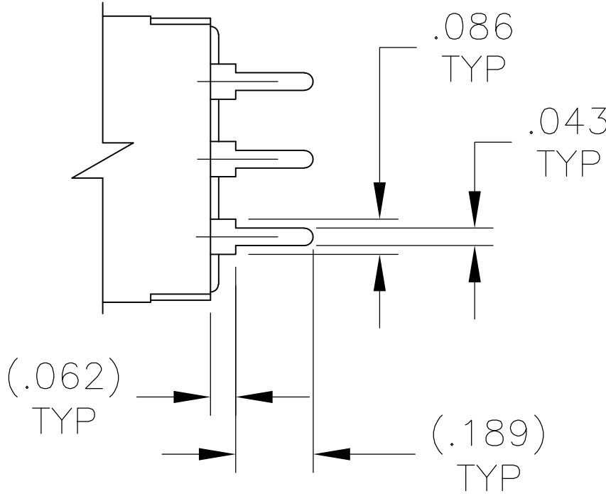
PC TERMINAL
